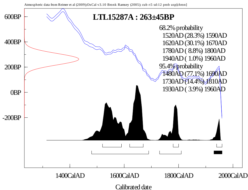
Figure 1. Calibration of the radiocarbon age of the sample LTL15287A.
