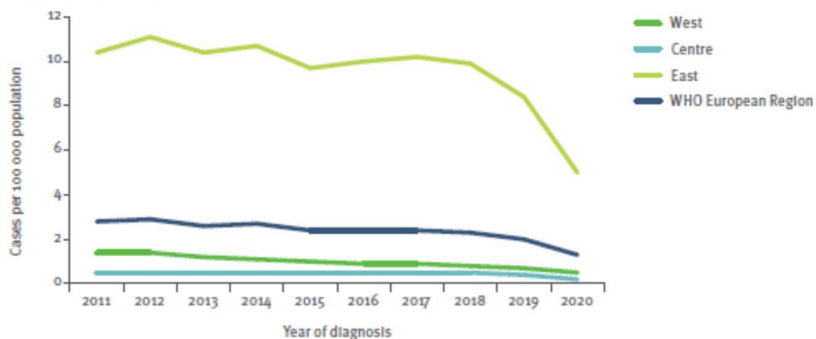
Figure 2.4: New AIDS diagnoses per 100 000 population, by geographical area and year of diagnosis, WHO European Region, 2011–2020
